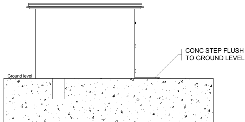
E.S.B. SUB-STATION LEFT SIDE ELEVATION
