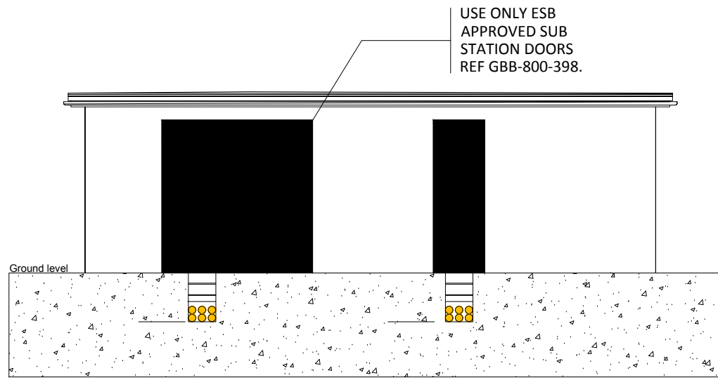
E.S.B. SUB-STATION FRONT ELEVATION
