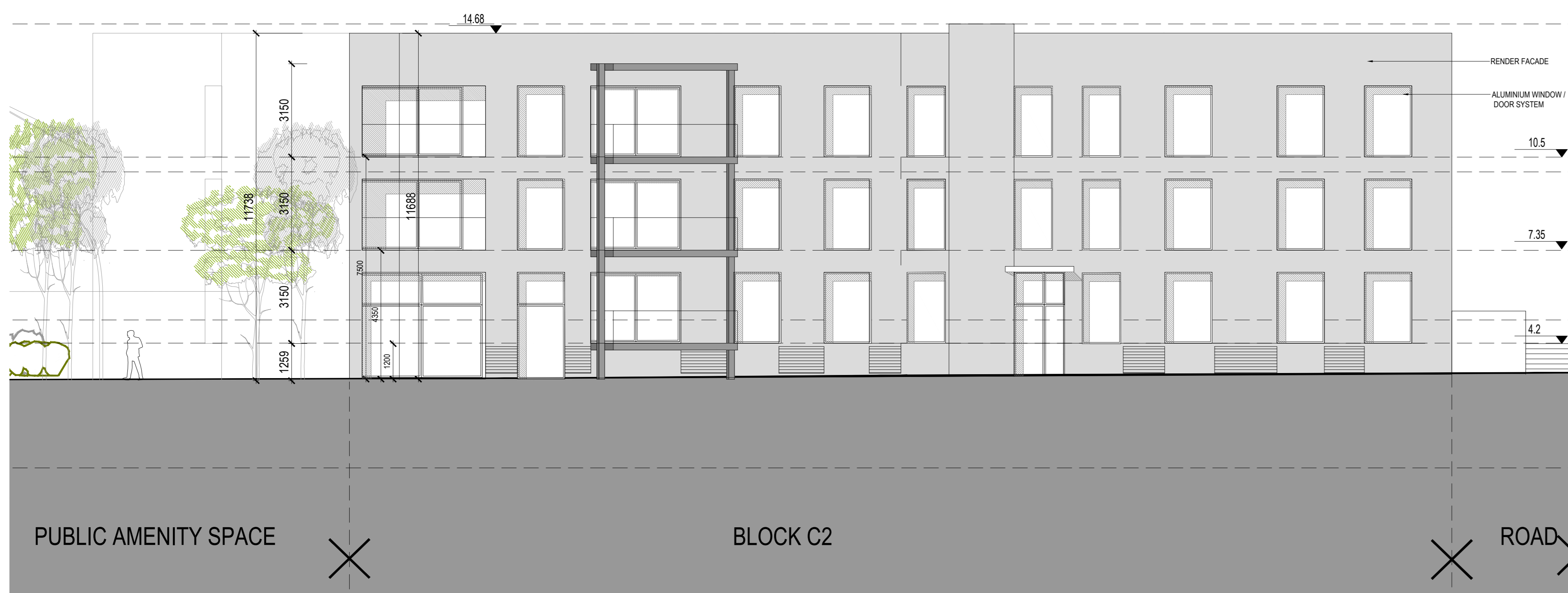
BLOCK C2 - NORTH ELEVATION
