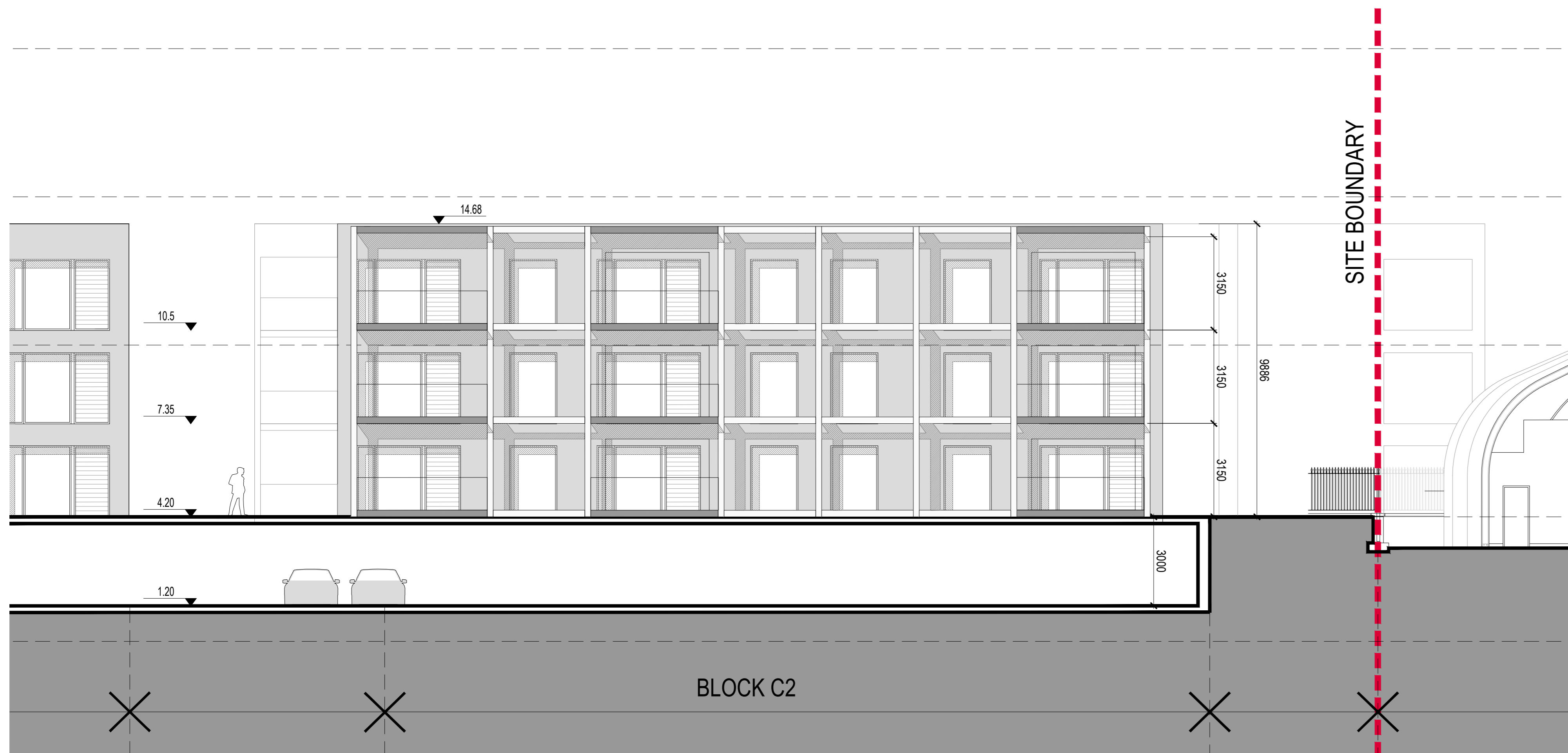
BLOCK C2 - SOUTH ELEVATION
