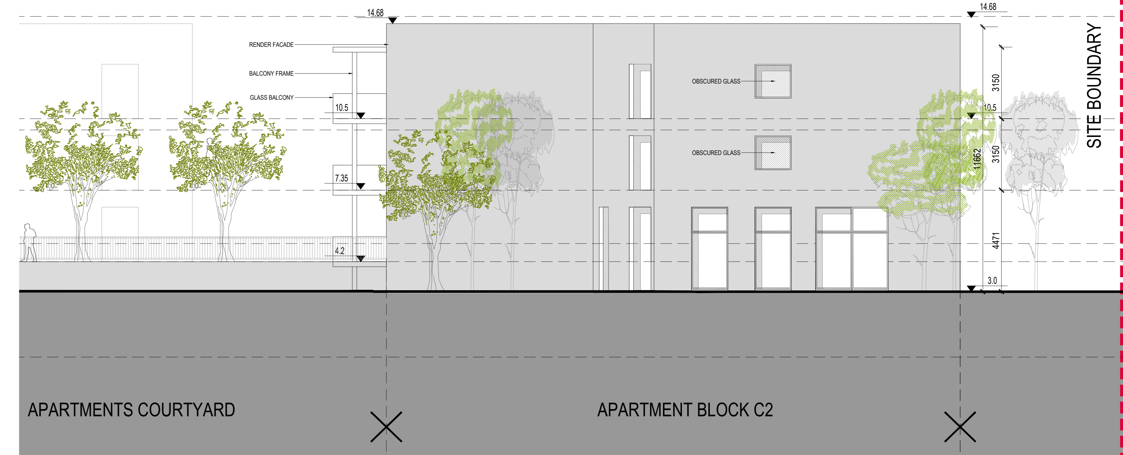
BLOCK C2 - EAST ELEVATION
